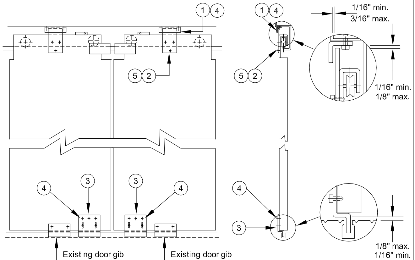
DOOR SAFETY RETAINER KIT FOR FIELD MOUNTING TO CENTRE PARTING LANDING DOOR.
