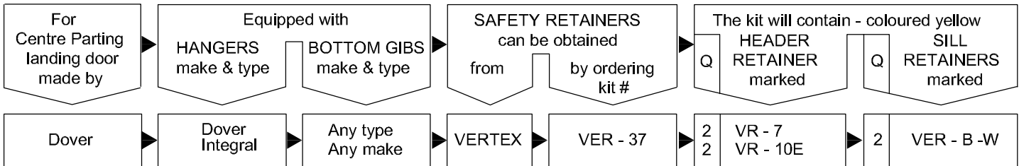
DOOR SAFETY RETAINER KIT FOR FIELD MOUNTING TO CENTRE PARTING LANDING DOOR.
